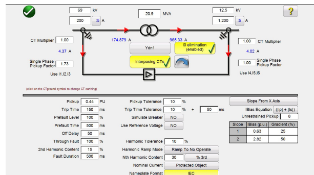
Figure 11 ANSI Transformer Differential Model
