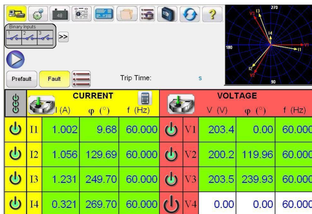
Figure 2 Color Accents when Selected Outputs are on (4 Channel unit shown)
