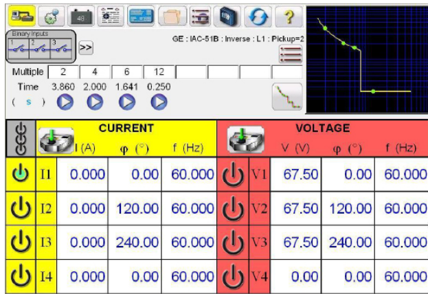
Figure 4 Timing G.E. IAC51B Overcurrent Relay (4 Channel unit shown)
