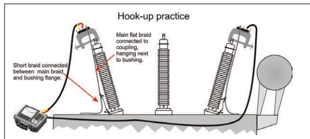
Solid connections using the C-clamps and the shortest braid method to connect the shield to ground, makes it possible to eliminate connection problems and cable loops that otherwise affect the measurement.
